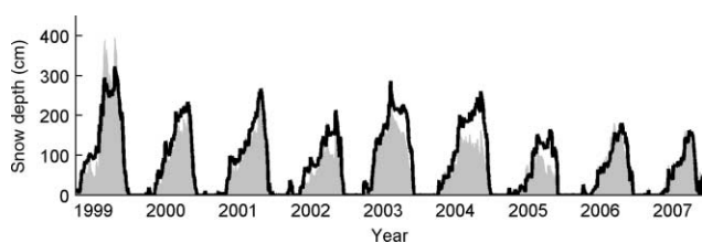
Figure 5 | Modelled snow depths (filled line) and interpolated snow depths (grey area) averaged over the flatter regions of the basin (slope angle less than 15^\circ ) between 2,000 and 2,500 m elevation.
